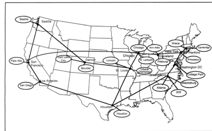
NSFNET Backbone 1992
